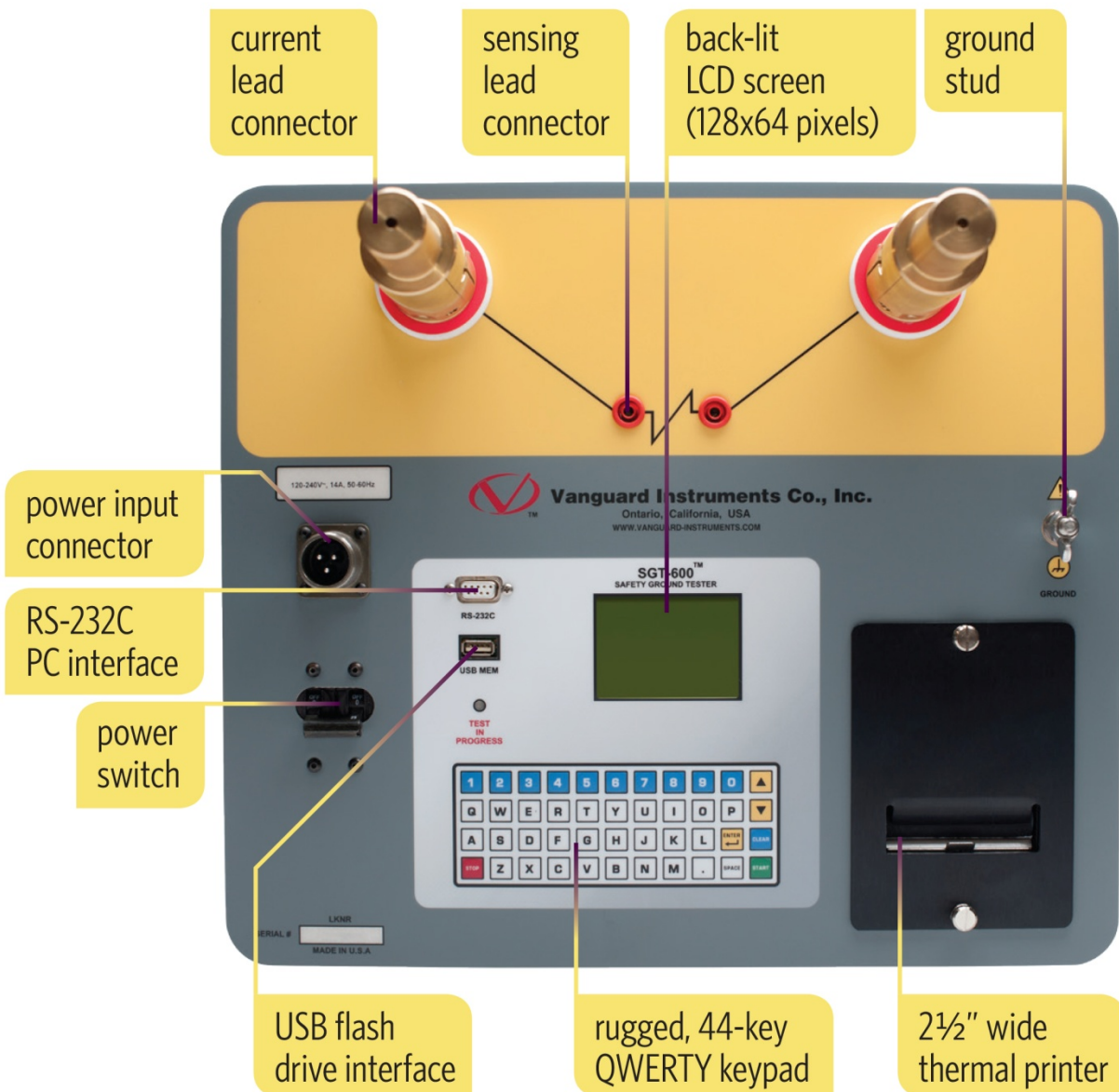
Figure 1. SGT-600 Controls and Indicators
