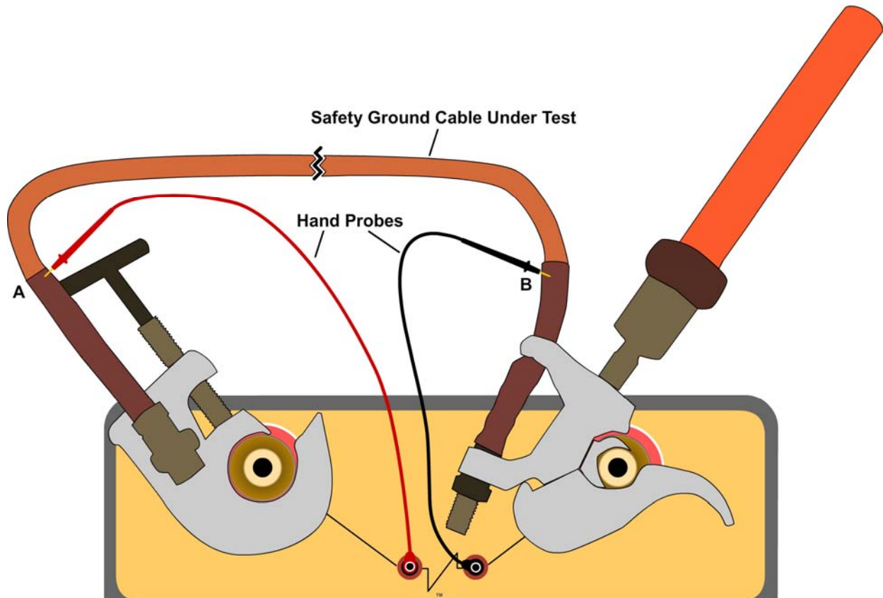
Figure 5. Performing a Diagnostic Test Between Points A and B
