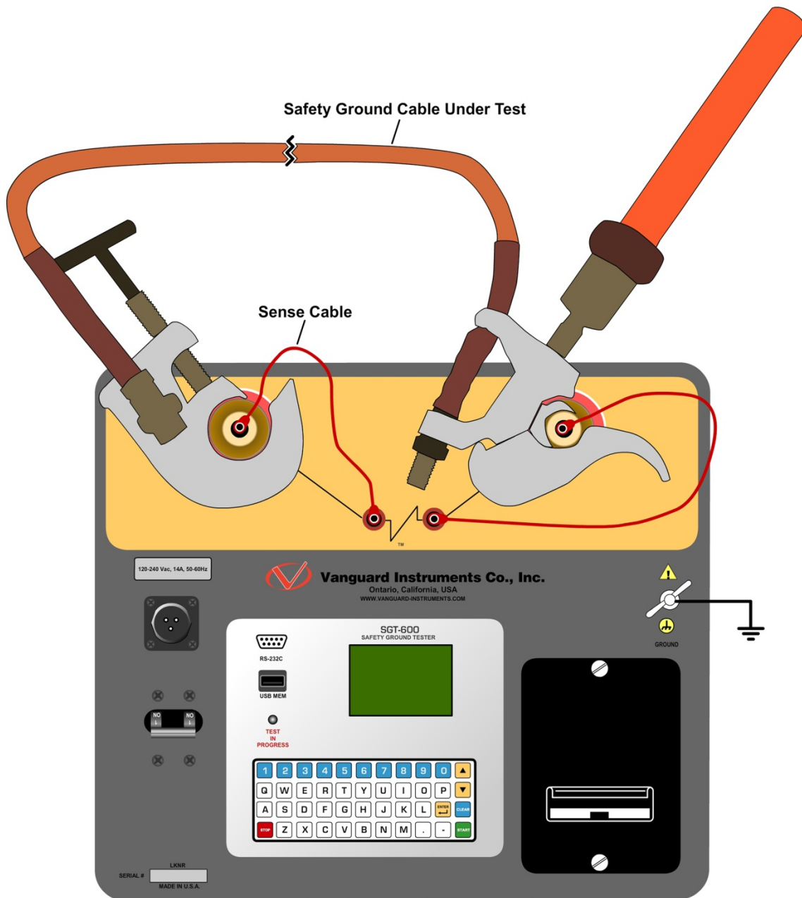
Figure 2. Typical SGT-600 Connection Diagram
